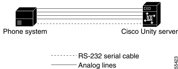
Figure 1-1 Connections Between the Phone System and Cisco Unity
